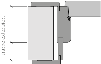
Stipite telescopico per tavolati superiori a cm 12 Telescopic jamb for wall thickness wider than cm 12
